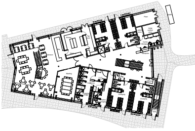
GROUND FLOOR PLAN 1 to 200 @ A1 1 to 400 @ A3
