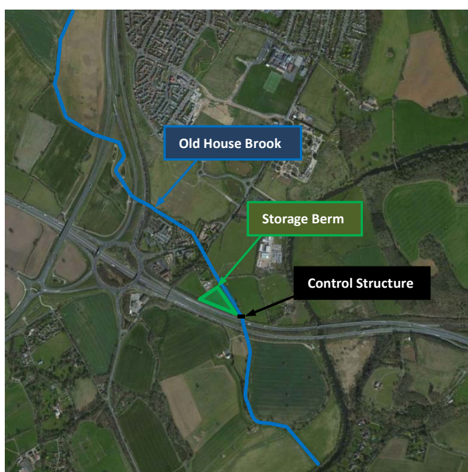
Figure 4a: Option 1 – Water storage within the site
